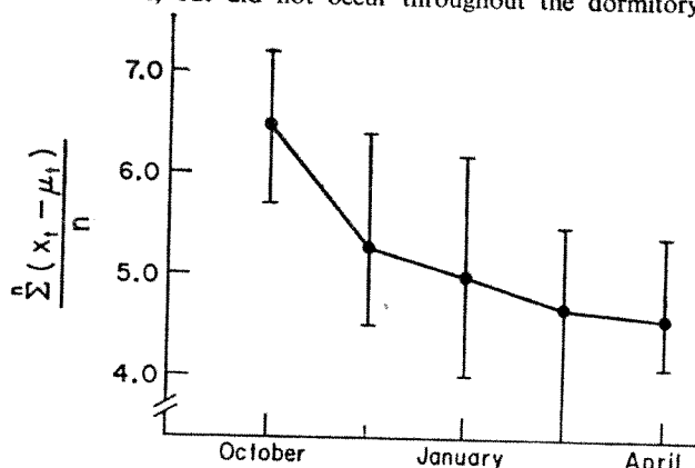
Fig. 1 The median individual mean difference from the group onset mean ( \frac{\sum (x_i - \mu_i)}{n} days) as a function of time. The asymptotic relation and non-overlapping confidence intervals 6 for the medians in October and late February, and October and April ( > 0.99 ), indicate an increase in synchrony for close friend groups.
